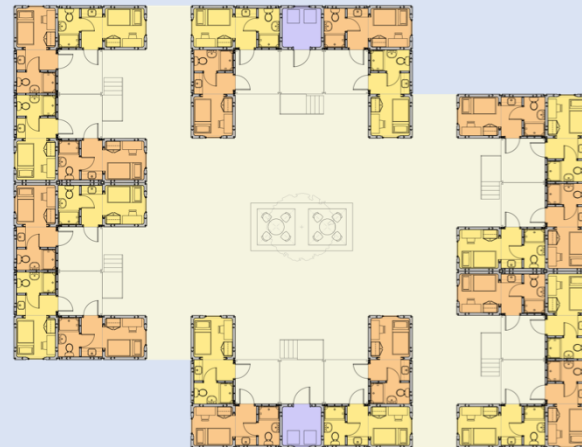
24 UNIT COMMUNITY CLUSTER
