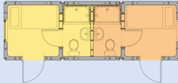
1.5 MODULE SHELTER UNIT
